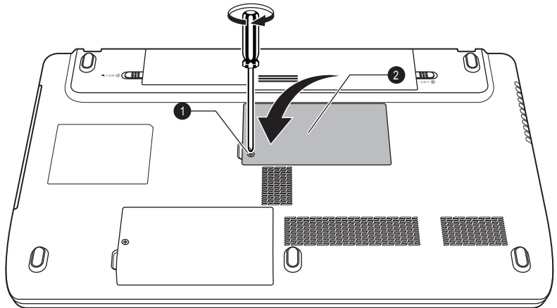
Figure 3-11 Seating the memory module cover (Satellite L770/L775/L770D/L775D/satellite Pro L770/L775/L770D/L775D)
